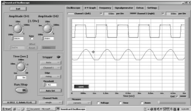
Figure 8.9 — If the text did not give it away, you would not have guessed this is the on-screen display of a no-hardware scope. The clue is the time scale, where you can see the input waveform frequency is close to 1 kHz — an audio frequency.
