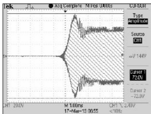
Figure A2.1 — Transceiver overshoot measurement with the Tektronix TBS1042.
