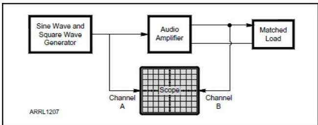
Figure 7.6 — This is the simplest test setup to look for problems with an audio amplifier. Notice that the load must be matched to the amplifier output to give valid results.
