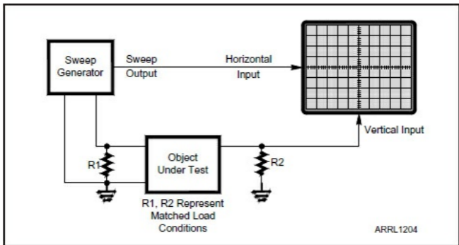
Figure 7.3 — A sweep generator and an oscilloscope can be used to see (and adjust) the passband of a filter, circuit or amplifier (the Object Under Test block).
