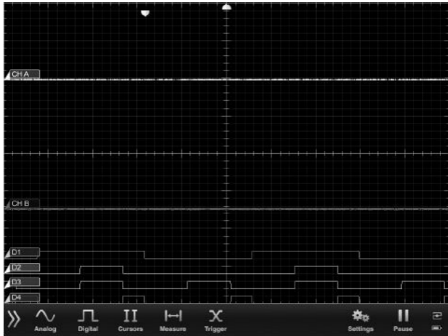
Figure A3.2 — The stages of a 4-flip-flop counter are connected to digital channels D1, D2, D2 and D4. Any digital channel can be selected to supply the trigger. In this screen shot channel D4 was selected.
