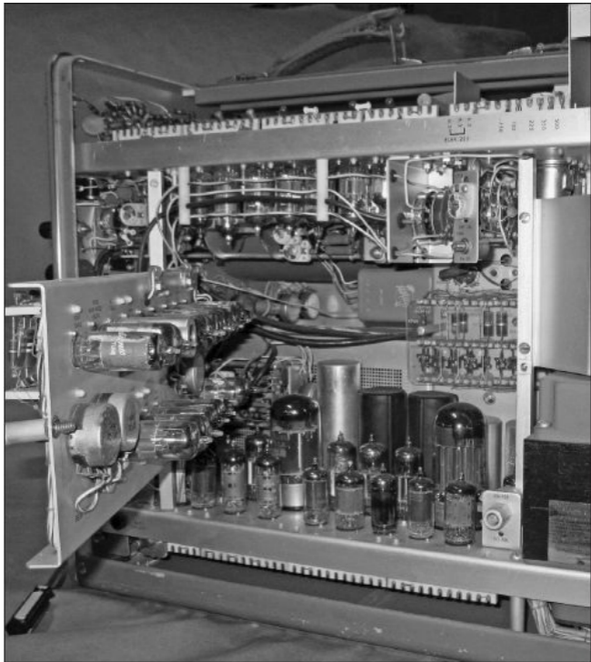
Figure 1.2 — Here you can see why the Tektronix tube scopes ran hot and consumed a great deal of space and power. This picture shows only part of the tube lineup.
