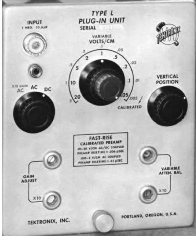
Figure 6.3 — This vintage Tektronix FAST-RISE plug-in front end provides very fast response to rising and falling pulse edges, useful for digital information where the pulse edges are important.
