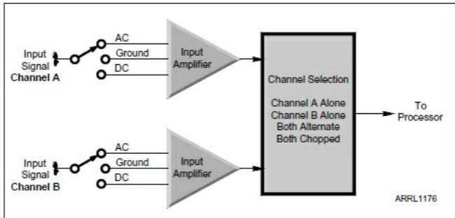
Figure 3.4 — An expanded block diagram for analog scopes shows two input channels, each preceded by a selection switch and followed by channel selection controls.
