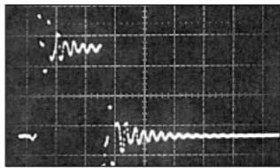
Figure 8.5 — If the sampling rate is too low, critical parts of the input waveform may be missed.
