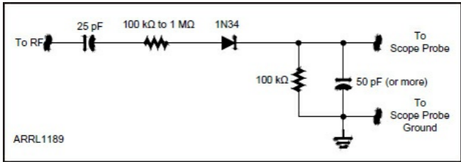
Figure 7.15 — This RF detector will produce a rectified envelope of your transmitted signal.
