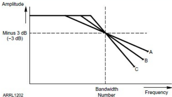
Figure 8.3 — Idealized vertical channel response, corresponding to the specified bandwidth. All three curves meet the specified bandwidth number, but with differing characteristics.
