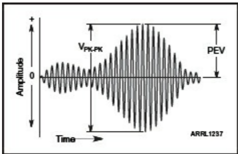
Figure 7.23 — The peak-to-peak voltage and peak envelope voltage (PEV) as seen on an oscilloscope screen.
