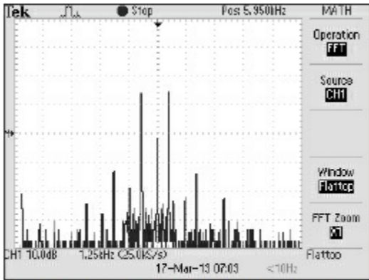
Figure A2.5 — Tektronix TBS1042 two-tone test FFT display using the same test setup as for Figure A2.4.
