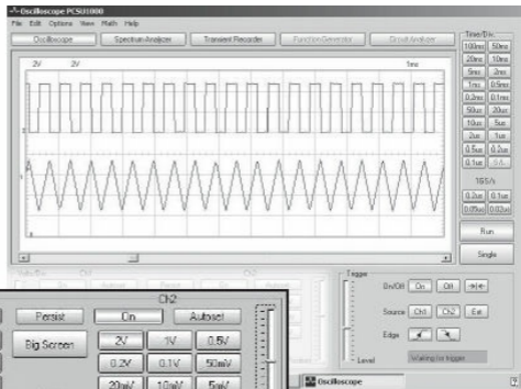
Figure 6.2 —This scope uses a mouse and an on-screen display to select the inputs as well as other functions. Channel 1 and Channel 2 are controlled independently via buttons in the lower left section of the display as shown in the closeup.
