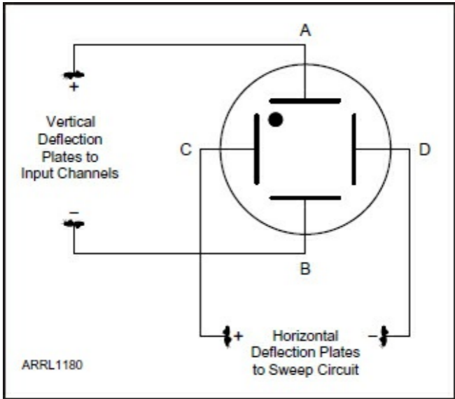
Figure 3.11 — The bias voltages shown here on the plates pull the electron stream toward the upper left corner of the screen.
