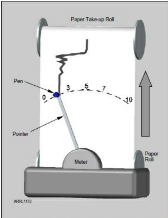
Figure 2.1 — A basic plotter, the predecessor to the oscilloscope. The paper moves under the pen of metal scribe so the trace shows the voltage or current as it changes. At zero volts the pen is on the left edge of the paper, and higher voltage moves the pen further to the right. The paper rolling along corresponds to the time axis.
