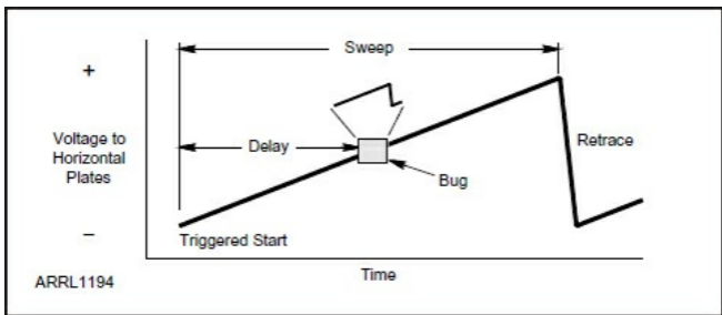
Figure 5.5 — When delayed sweep is selected, a point on the trace — often called a bug — is intensified to show what portion of the trace will be expanded.
