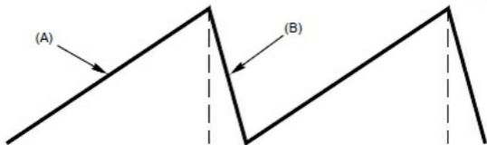
Figure 3.6 — The sweep voltage labeled A sends the beam across the screen from left to right. Waveform section B retraces the beam back to the left. During this retrace time the electron beam is cut off. In a digital scope the retrace time is the time to reset the counter and is reduced to close to zero.
