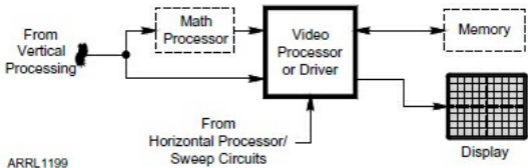
Figure 5.10 — Digital oscilloscopes are best shown by this functional block diagram. The hardware is actually a microprocessor, digital memory and video driver — in other words, part of a personal computer or equivalent.
