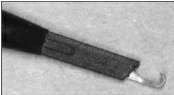
Figure 4.6 — Typical probes have some sort of hook or grab mechanism to fasten onto a circuit lead or test point.
