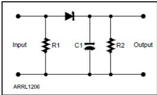
Figure 7.5 — If you need dc from the test setup, a simple rectifier circuit will work. C1 is 0.01 \mu\text{F} for audio frequencies or 100 pF for RF. R1 and R2 are matching resistors as needed. You may have to make output capacitor C1 larger or smaller depending on the signal.
