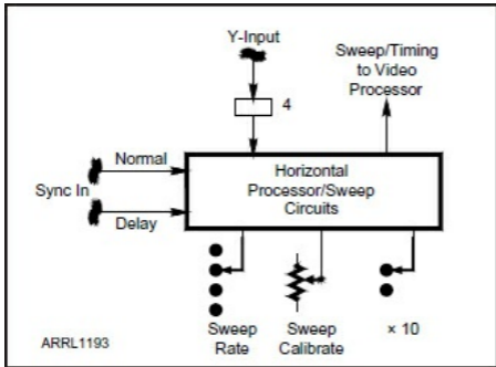
Figure 5.4 — The horizontal section of a scope has the same functions whether implemented in hardware, software, or a combination of both.
