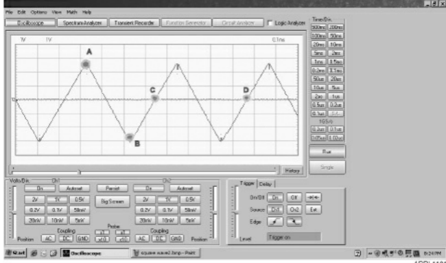
Figure 3.14 — The digital processor can detect points A, B, C and D and automatically calculate maximums, minimums, RMS, average, period and other waveform parameters.
