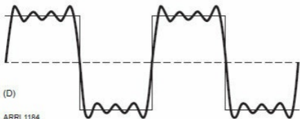
Figure 4.2 — The actual equation for a square wave sums a sine wave at the original frequency at a given amplitude, plus a second sine wave at \frac{1}{3} the original amplitude and 3 times the frequency, plus another sine wave at \frac{1}{5} the original amplitude and 5 times the original frequency, and so on.
