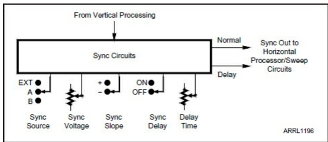
Figure 5.7 — On some oscilloscopes, the sync controls have other names. The objective of this section is to select a point on a waveform and generate a pulse to start the horizontal sweep.
