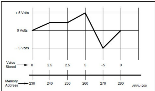
Figure 5.11 — If you were able to see into the memory, the stored values would consist of a set of 1s and 0s — programming tools would show them as hex values. The memory addresses would also show as hex values.
