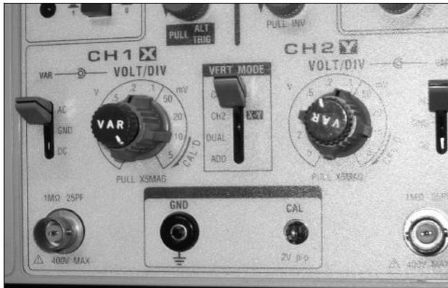
Figure 7.1 — Channel 1 is calibrated (VAR knob fully clockwise, in the CAL'D position), so the VOLT/DIV setting is correct. Channel 2 is not calibrated (VAR not fully clockwise), which can lead to false measurements.
