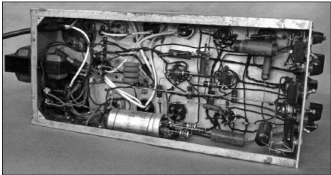
Figure 2.B — The inside of W1GIG's scope. This is the wiring technique typical of a ham 50 years ago.
