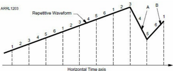
Figure 8.6 — The repetitive waveform in this figure is shown drawn against a time axis. If the sampling rate is too low, only the waveform points labeled 1 will be seen, and the true shape of the waveform in the areas labeled A and B will be missed — corresponding to the missed points in Figure 8.5. If the sample points are repeated, but slightly delayed in time (points labeled 2) in a second sweep, and 3 in a third sweep, and so on — the displayed waveform will more and more assume its true shape. In this figure a set of 6 samples are shown, requiring 6 sweeps to more accurately show the waveform shape.
