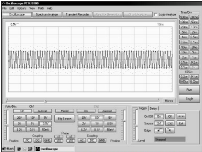
Figure 7.9 — A constant, single tone input to an SSB transmitter produces this uniform picture. If there were noticeable carrier (not enough carrier suppression), the envelope would not be flat.
