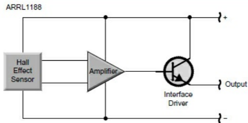
Figure 4.10 — The Hall Effect sensor puts out a tiny voltage, so most commercial units include a preamplifier. The connection from the probe end to the scope must therefore include power wires and sometimes control wires.
